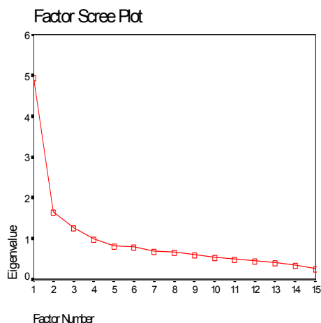
Figure 1. Graphic showing the number of factors versus self values
